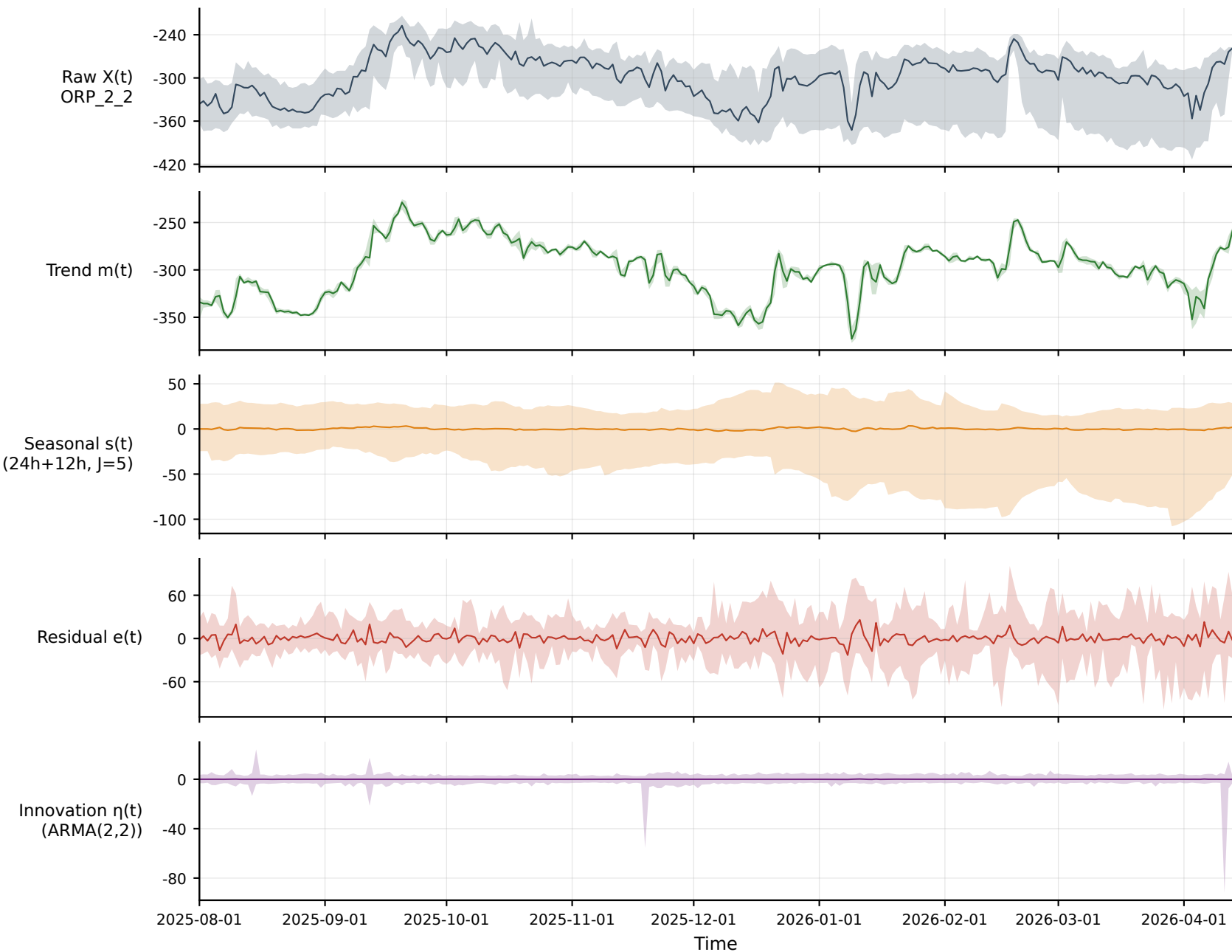
Full-span daily overview — ORP_2_2 (pre_anoxic_front, min) [2025-08-01~2026-04-13]
